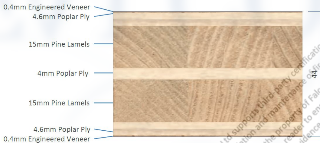
Fig. 3 – Cross section through Type A door blank design
