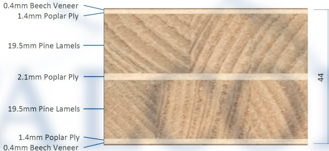
Fig.2 – Cross section through Type B door blank design
