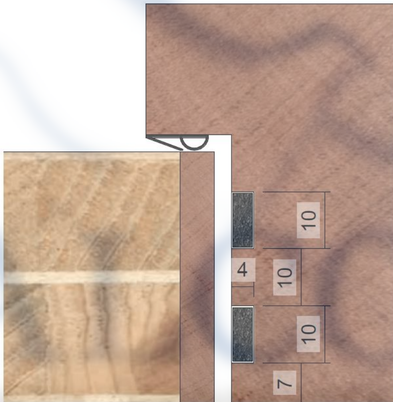
Fig. 10 – Frame profile indicating the required position of the perimeter intumescent seals (dimensions in mm)
