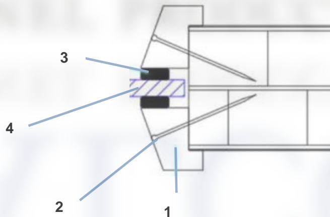
Fig 8: Cross section of tested and approved Sealmaster glazing system (item 4 detailed below)
