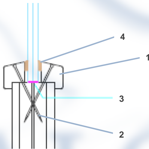
Fig 9: Cross section of tested and approved glazing system
